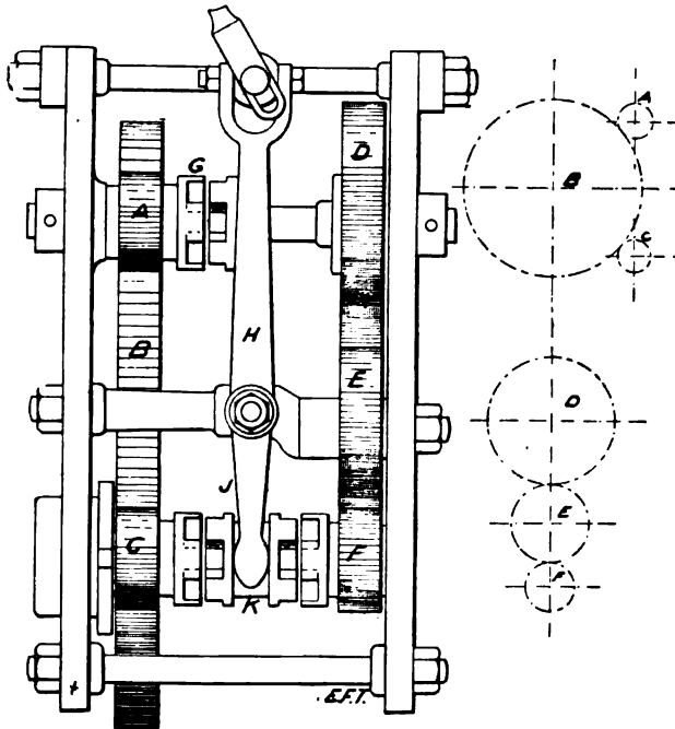
FIG. 352.—The Didier Two-speed Tricycle Gear. A rotating clutch pulley, K , slides on a feather on the main shaft, its position being shifted to the right or the left by the arm, J , of the lever, H , actuated by the handle as shown at the top of the figure. When it is moved to the left it engages the spur pinion, C , which meshes with the main drive gear, B , thus driving the cycle at the first or lowest speed. When it is moved to the right it engages the spur pinion, F , the rotating clutch, G , also engaging the pinion, A , on the second shaft, so that F drives D through E and B through A , thus giving the second speed. The relative position of the six gears is indicated by the diagram to the left of the figure.
